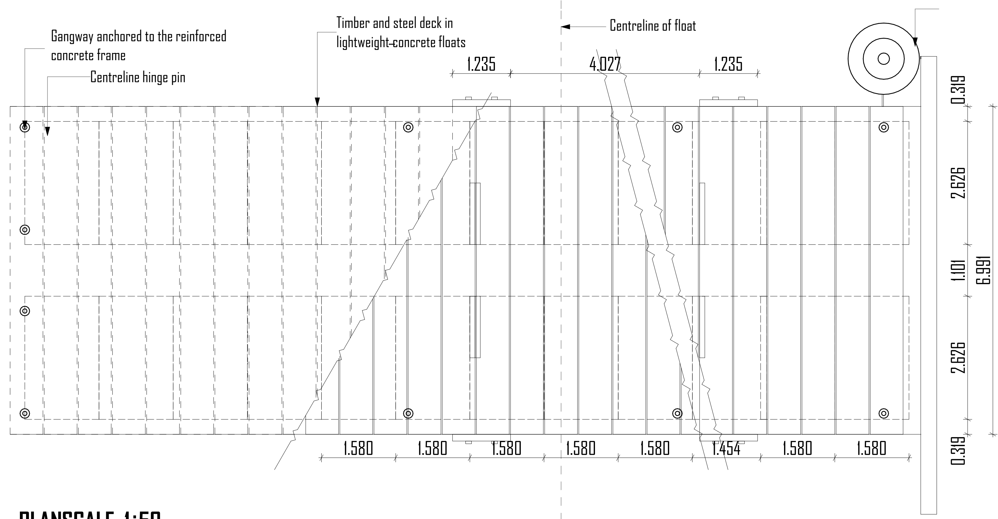
PLANS SCALE 1:50
