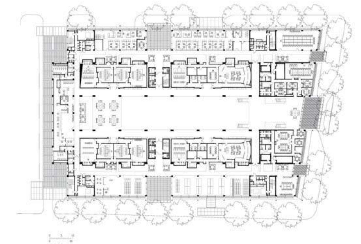
PLAN LAYOUTS
