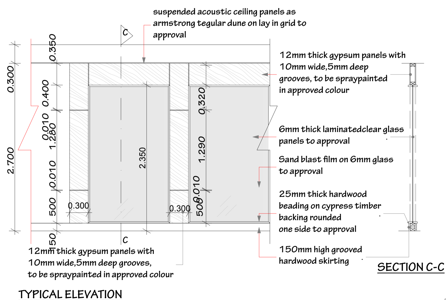
TYPICAL GYPSUM PARTITION DETAILS (PROCUREMENT OFFICES)
