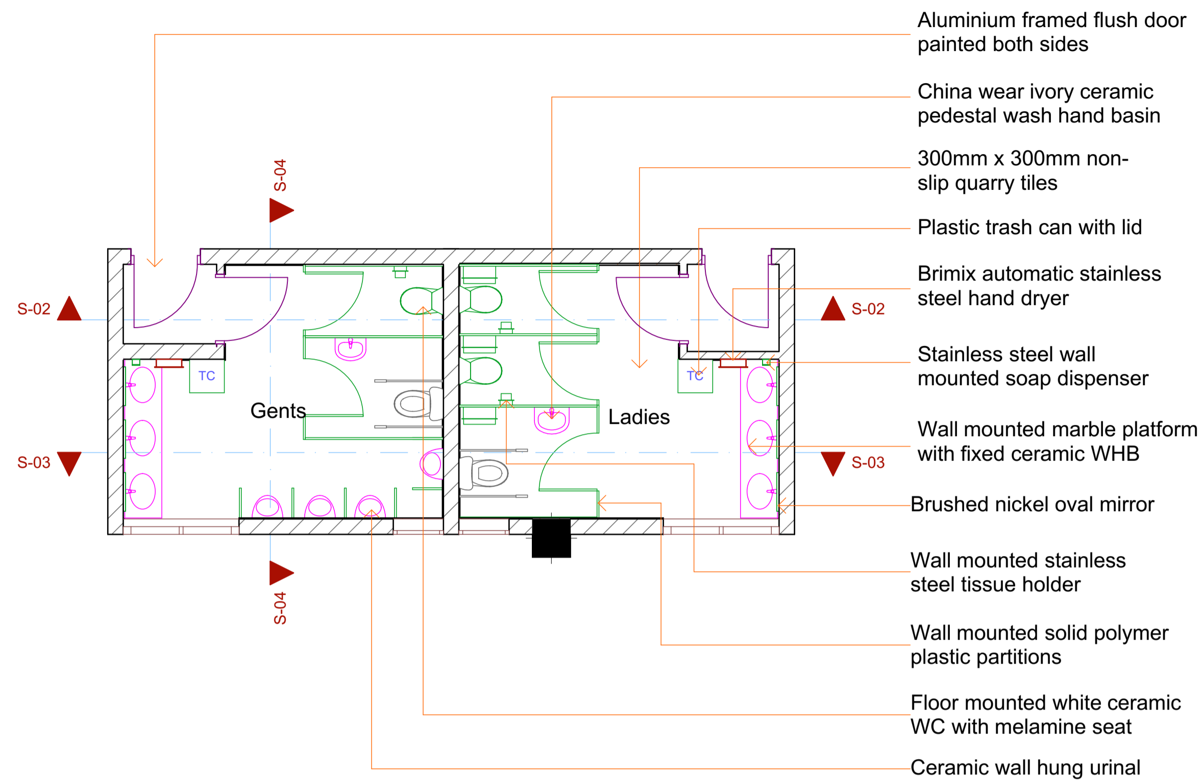
Floor plan
