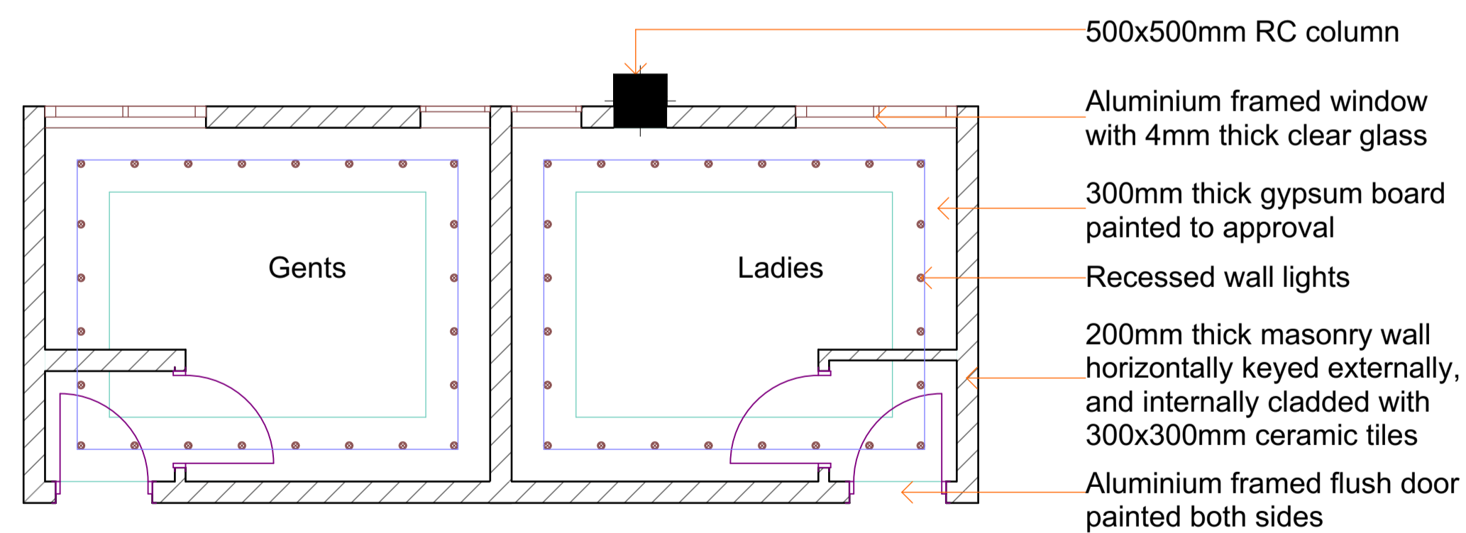
Ceiling plan
