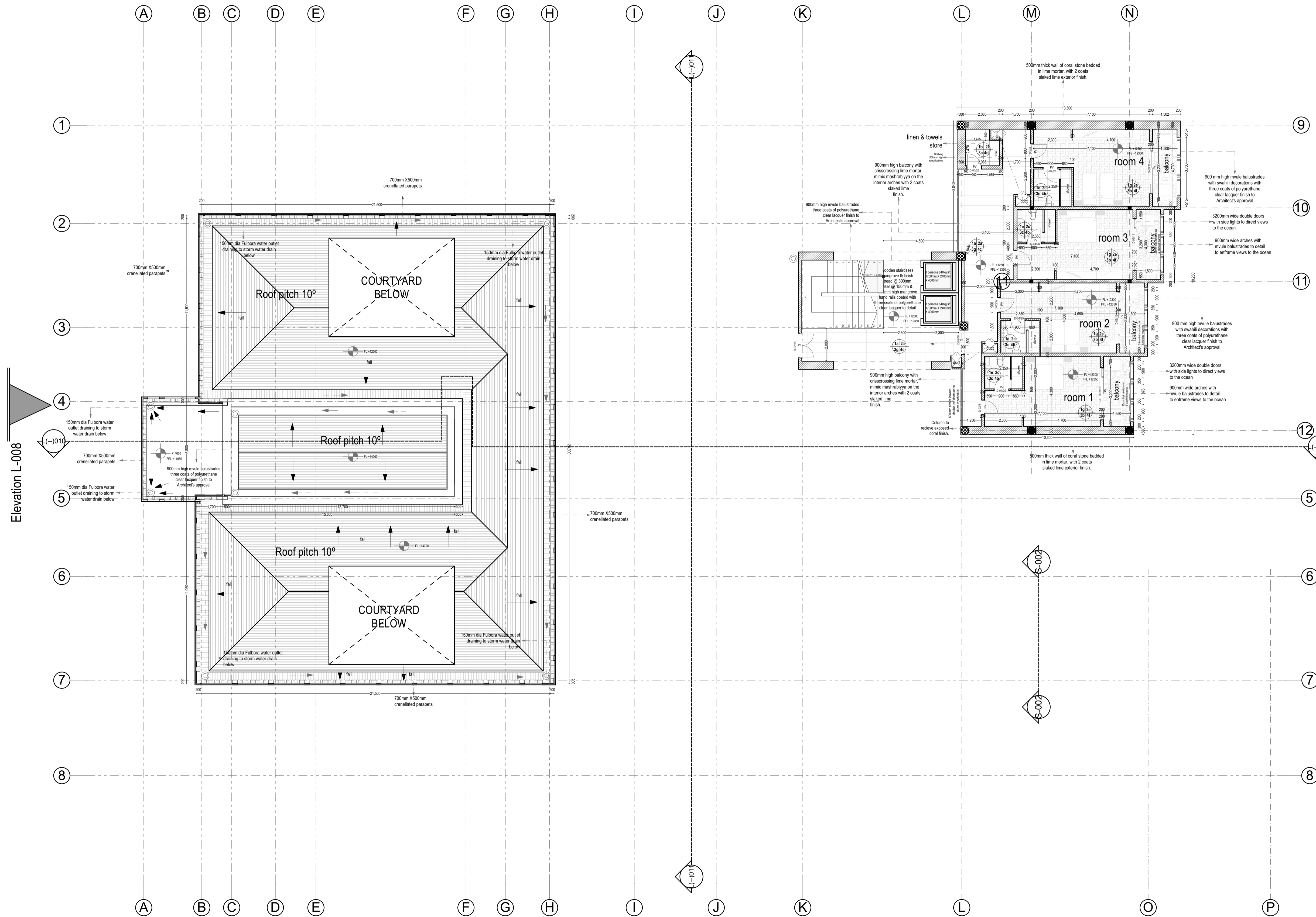
Third Floor Plan L(-)005
